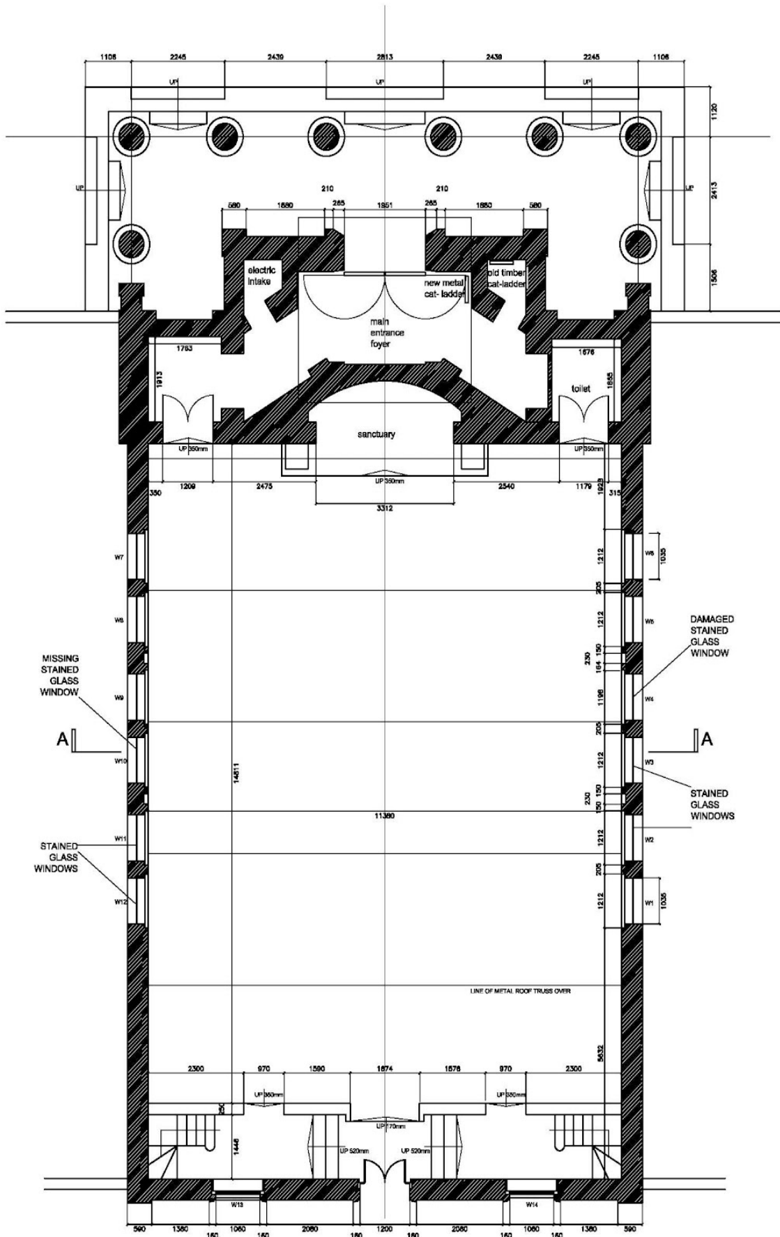
GROUND PLAN
